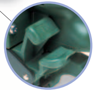
Operation levers The ergonomically arranged tensioning and sealing levers permit a quick operation of the tool.
